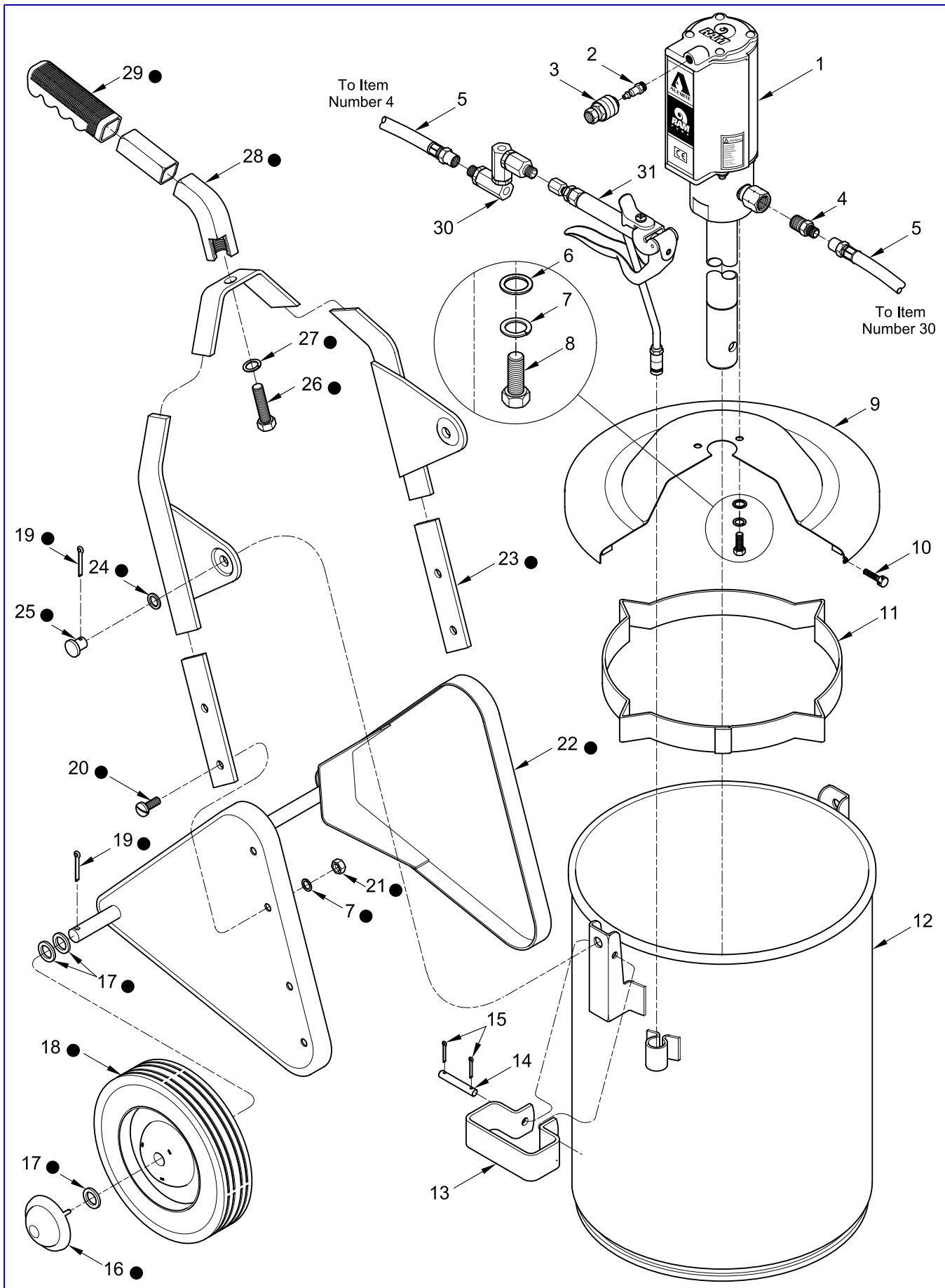
Figure 2 High-Pressure Portable Pump Models 9911-A and 9911-B - Exploded View
