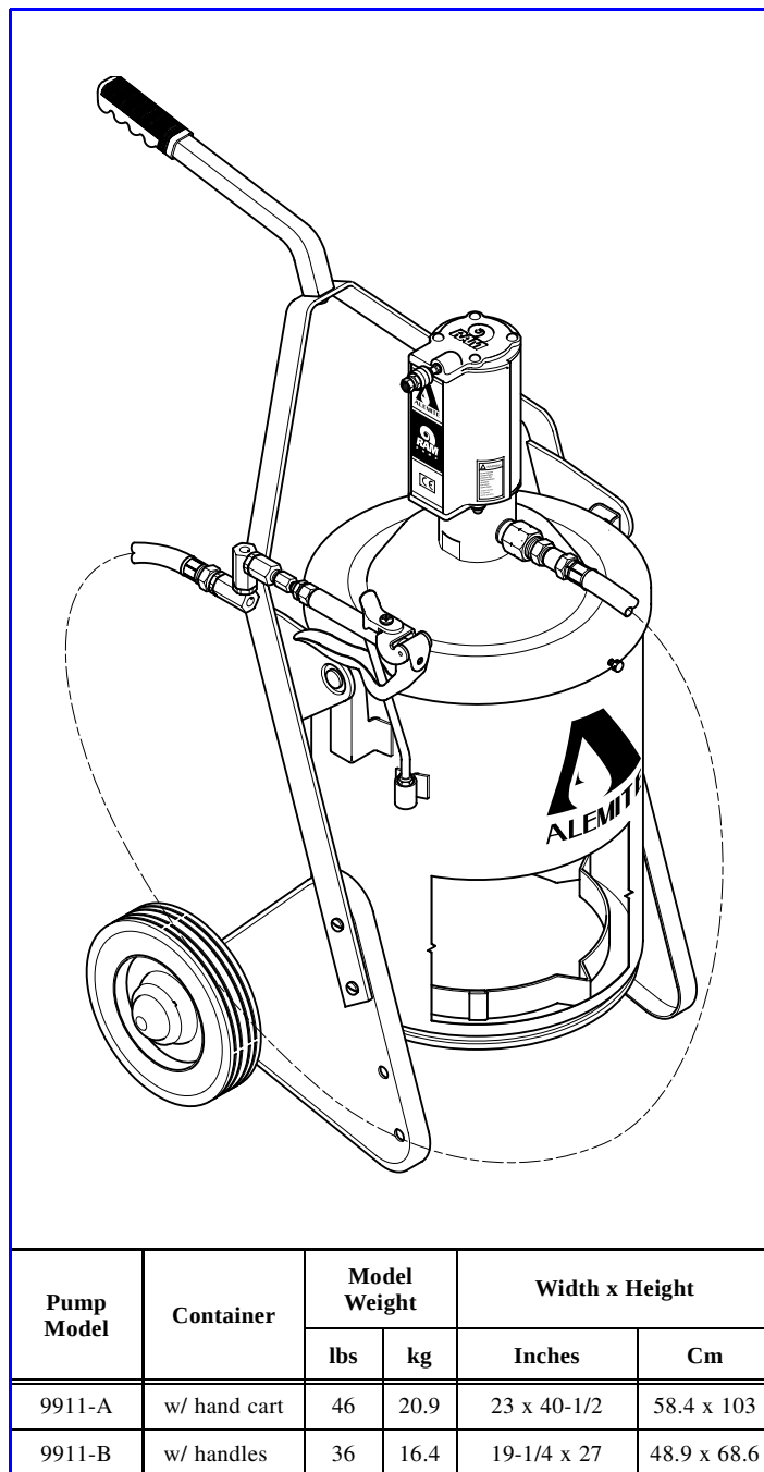
Figure 1 High-Pressure Portable Pump Models 9911-A and 9911-B - Model 9911-A Shown
